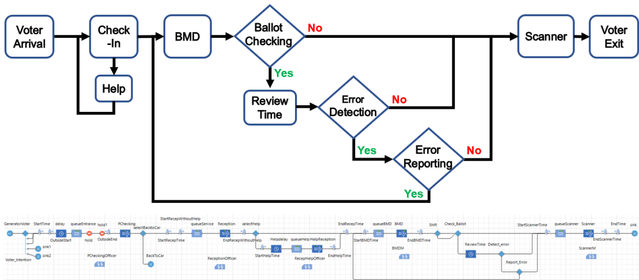
Figure 4: Voting Process.
