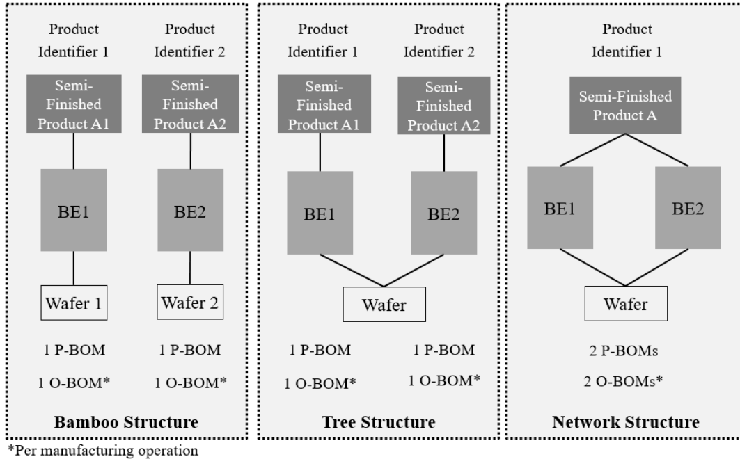
Figure 3: Example of product structure representations in the semiconductor industry: bamboo, tree and network ( BE stands for back-end manufacturing processes ).
